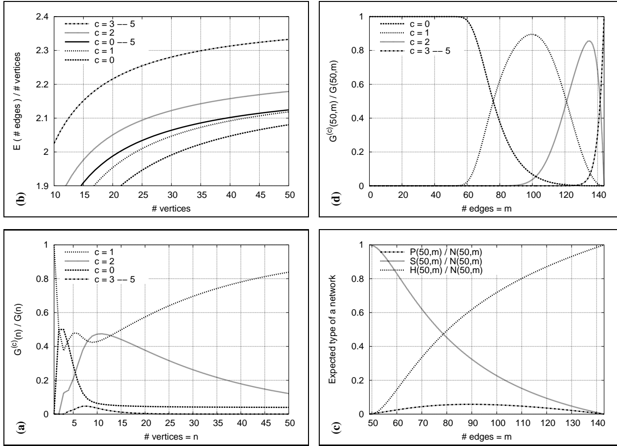
Fig. 2. Some counting results. (a) Expected connectivity, n running (b) Edge density, n running (c) Expected type of a network, m running (d) Expected connectivity, m running
